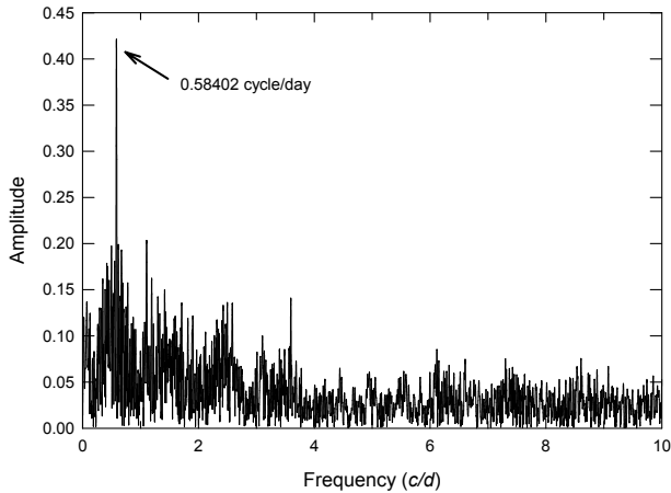
Figure 2. Amplitude spectra of P_1 using Period04
