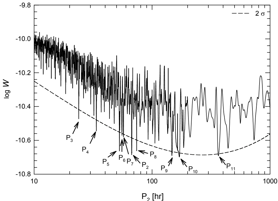
Figure 4. W vs. P_2 for the 3rd order 2-dimensional Fourier series with P_1 = 82.2 h (solid line) and the 2\sigma range of W (dotted line).
