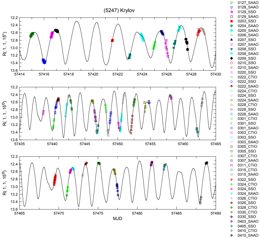
Figure 5. The 2-dimensional Fourier series (solid line) with P_1 = 82.188 h and P_2 = 67.13 h, plotted over Figure 1.
