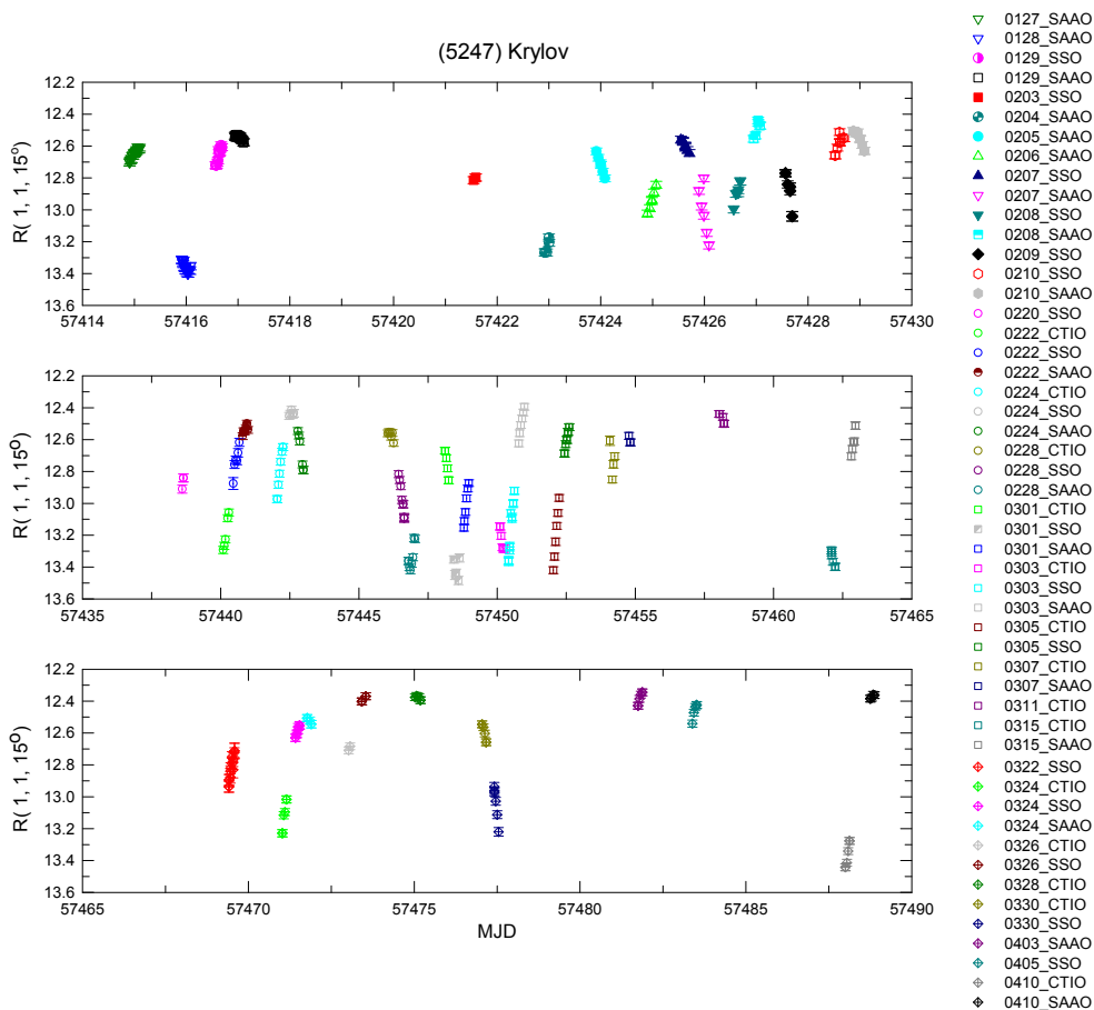
Figure 1. Geo- and heliocentric distance and solar phase angle-corrected R-band light curve of (5247) Krylov.
