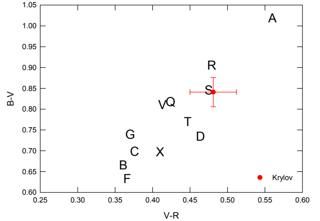
Figure 8. The V-R vs. B-V two-color diagram of different taxonomic types. Characters and red dot are the same as in Figure 7.
