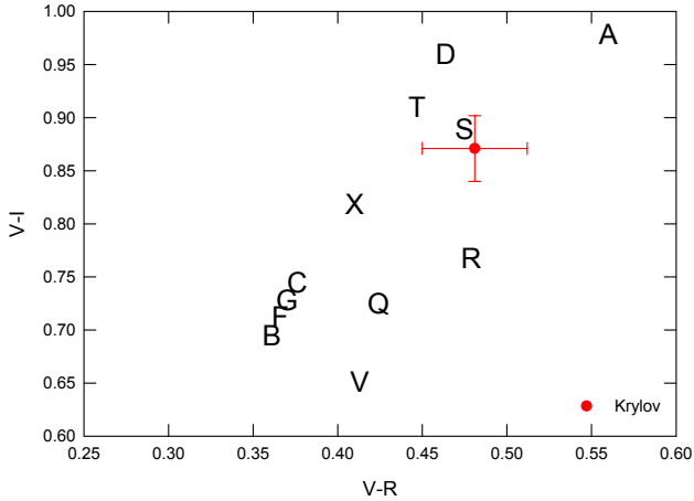
Figure 7. The V-R vs. V-I two-color diagram of different taxonomic types. The assorted characters represent different taxonomic types according to Dandy et al. (2003). The red dot represents (5247) Krylov.
