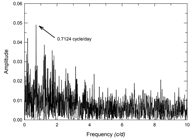
Figure 3. Amplitude spectra of P_2 using Period04
