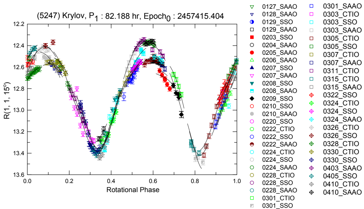
Figure 6. Same as Figure 5 but in the phase domain, using the period P_1 = 82.188 h.
